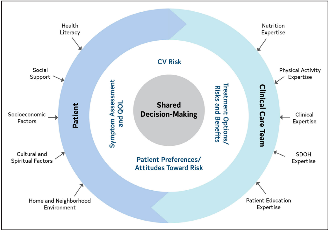
Figure 4. Domains to Consider When Seeing a Patient With CCD. CCD indicates chronic coronary disease; CV, cardiovascular; QOL, quality of life; and SDOH, social determinants of health.
